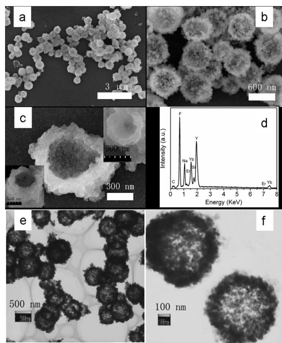
Figure 2. SEM and TEM images with different magnifications (a, b, c, e, f) and the EDS (d) spectrum of NaYF 4 :Yb 3+ , Er 3+ HNS prepared under hydrothermal treatment at 160 °C for 24 h with a 5 wt.-% concentration of the aqueous PEI solution. Inset: SEM images of the broken spheres.
