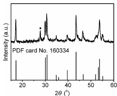
Figure 1. XRD pattern of the NaYF 4 :Yb 3+ , Er 3+ phosphors prepared by hydrothermal treatment at 160 °C for 24 h with a 5 wt.-% concentration of the aqueous PEI solution. The black dot (•) represents the peak (28.42) of the \alpha phase.
